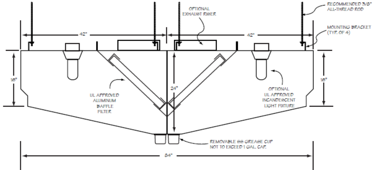
SECTION VIEW -- TYPICAL INSTALLATION
